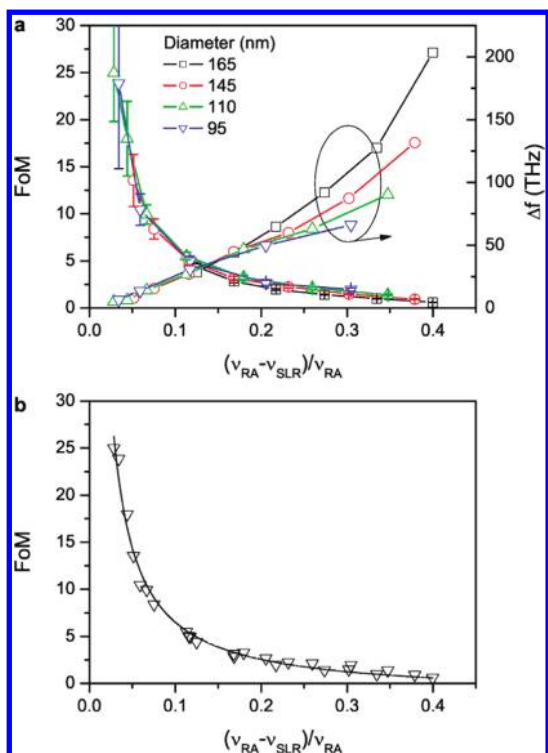
Figure 4. Measured FoM for different gold nanoparticle arrays and fit of the experimental data. (a) Experimental FoM ( \partial\lambda/\partial n )/ \Delta\lambda and the full width at half-maximum \Delta f of surface lattice resonances as a function of the parameter \delta = (v_{RA} - v_{SLR})/v_{RA} for particle arrays with diameters 95, 110, 145, and 165 nm, height 50 nm, and lattice constant a = 300, 350, 400, 450, 500, 550, and 600 nm. (b) The solid line is a fit to the experimental data (symbols) indicating a reciprocal scaling of the FoM with \delta .
